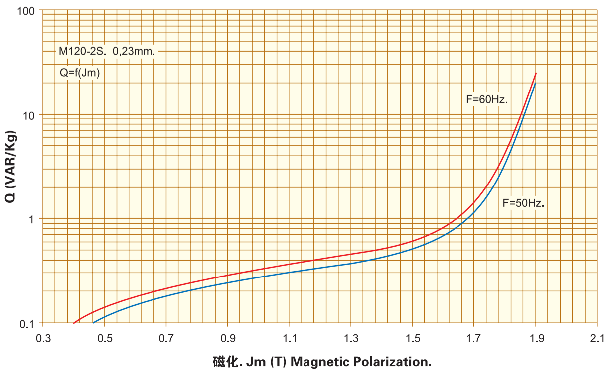
无功功率. Reactive Power. (VAR/Kg) Q=f(J_m) 0,23mm. M120-23S
