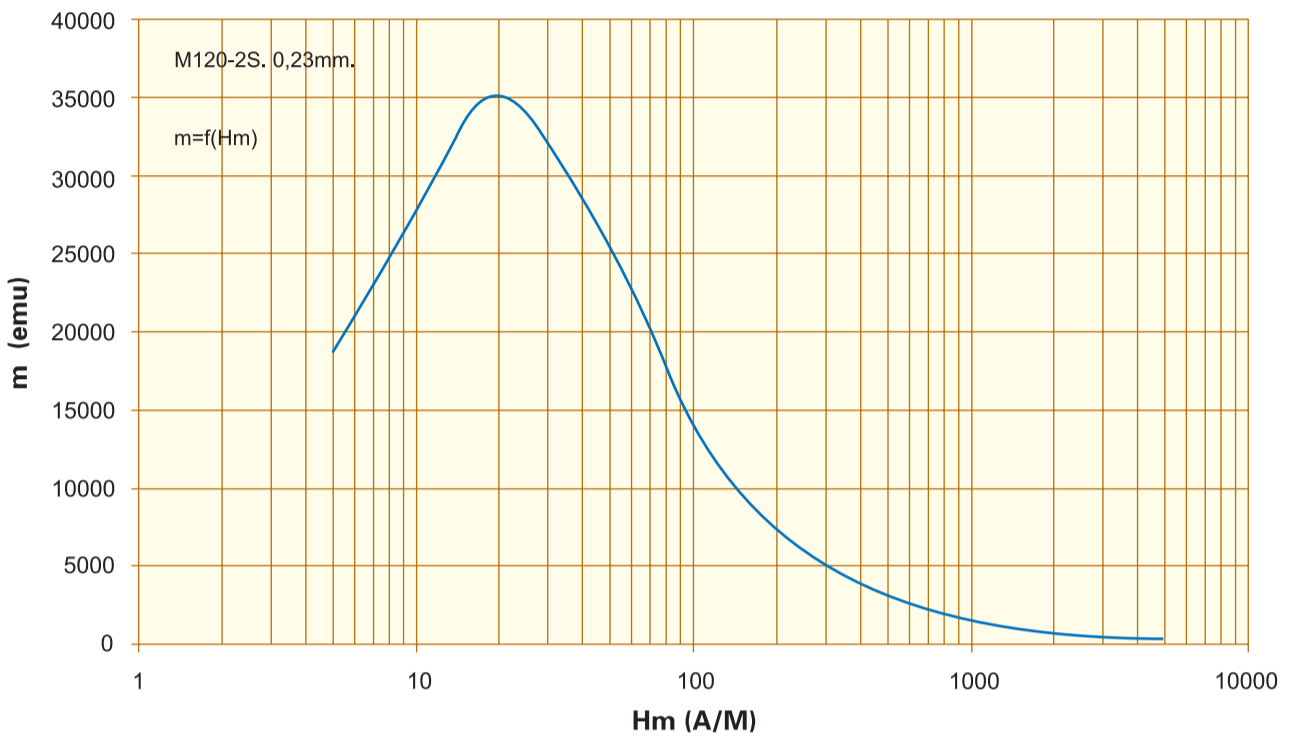
相对导磁率 Relative peak permeability. m=f(H_m) , F=50\text{Hz} , 0,23mm. M120-23S
