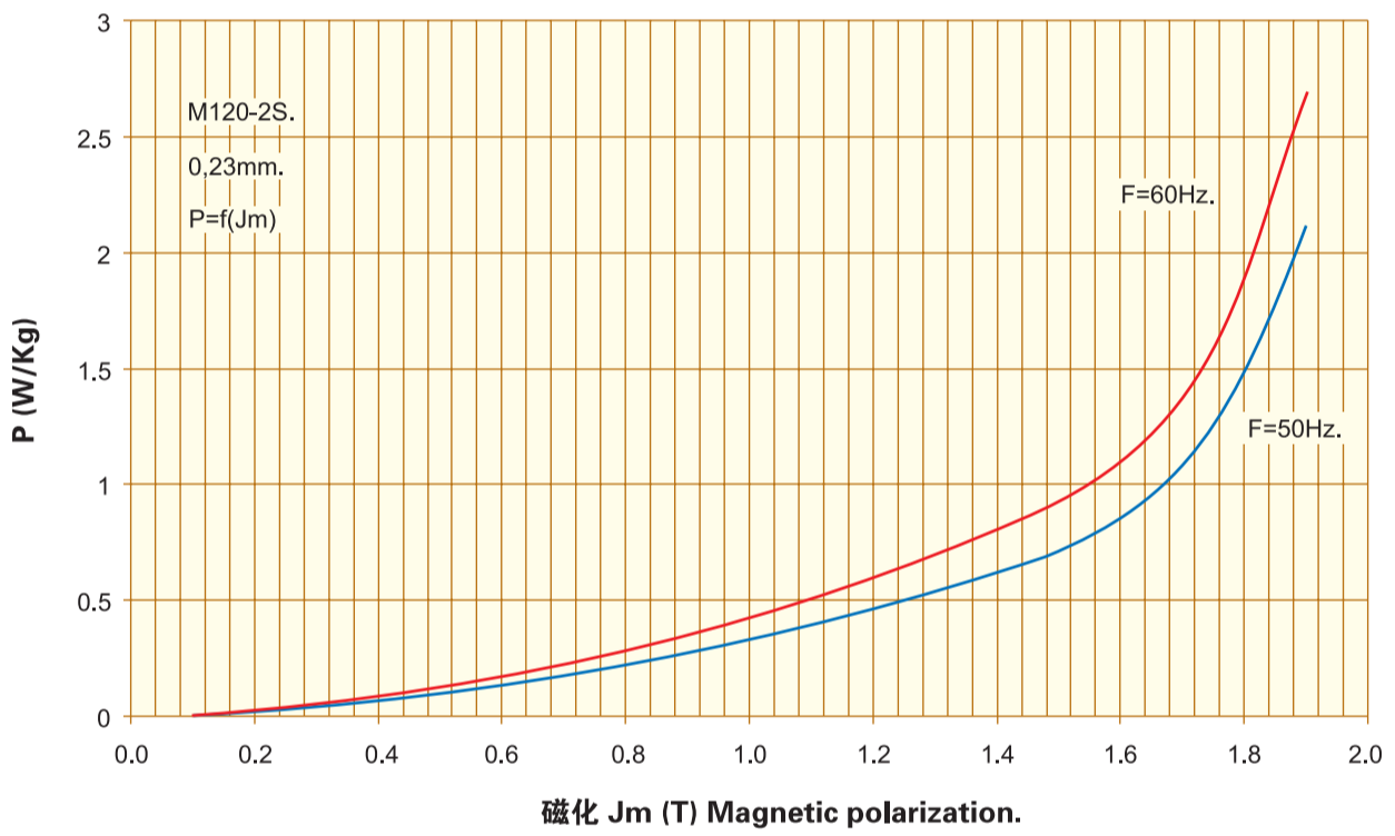
磁损耗. Specific Core Loss. P=f(J_m) 0,23mm. M120-23S
