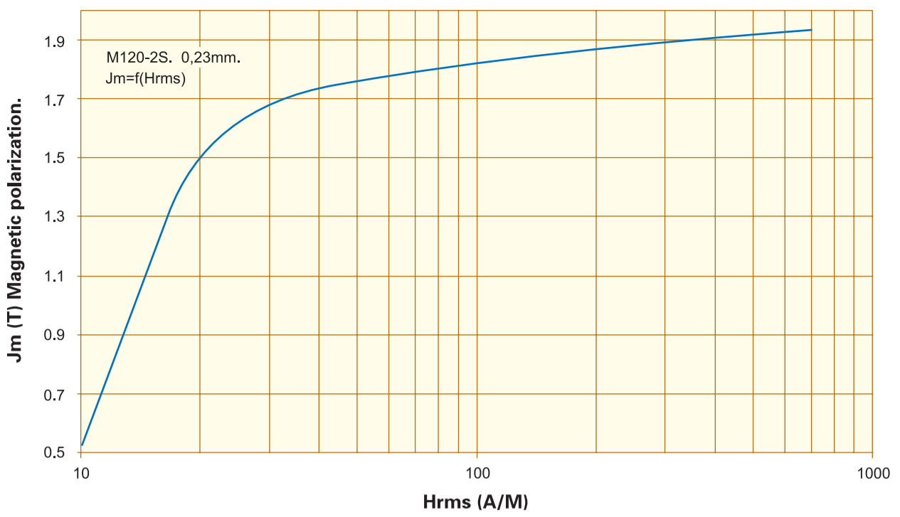
磁化曲线 Magnetic polarization. J_m=f(H_{rms}) 0,23mm. M120-23S
