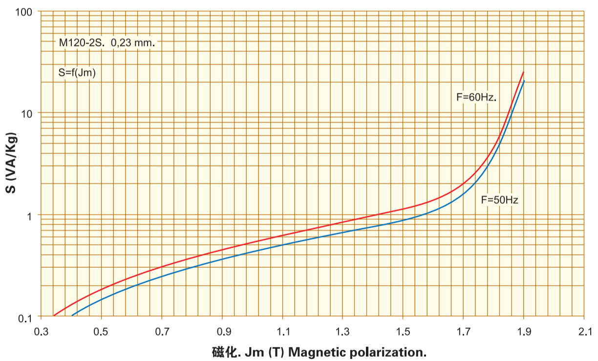
激磁功率. Exciting Power. S=f(J_m) (VA/Kg) 0,23mm. M120-23S.
